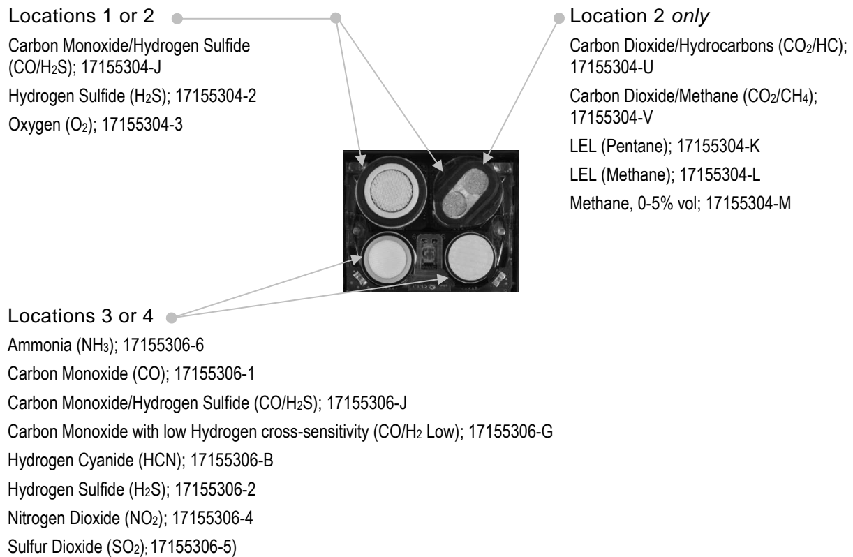
Figure 2.1.B Sensor compatibility and installation locations for the Ventis Pro5
